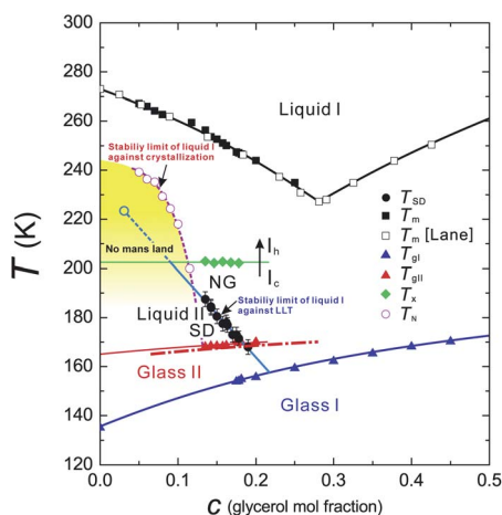
Fig. 15 Glycerol concentration vs. temperature ( c - T ) state diagram of water–glycerol mixtures. T_{SD} : LLT spinodal temperature (black filled circles); T_{gl} : the glass transition temperature of liquid I (blue filled triangles). For pure water ( c = 0 ), we use the widely accepted value of 136 K ° for T_{gl} ; T_{gII} : the glass transition temperature of liquid II (red filled triangles). Dot-dashed line indicates T_{gII} of pure liquid II without ice I_c , provided that liquid II contains \phi_c = 17\% of ice I_c , which should result in the increase in the glycerol mole fraction of liquid II by 6.4%; T_H : the homogeneous nucleation temperature (violet open circles) measured for the cooling rate of 100 \text{ K min}^{-1} ; T_c : the transition temperature from ice I_c to I_h , which was determined by microscopy observation (green filled diamonds); T_m : the melting (liquidus) temperature (black filled squares: our data; open squares: the data of Lane 198 ). We make a linear extrapolation of T_{SD} to estimate the position of a hypothetical critical point (CP) (light blue open circle), since we cannot access T_{SD} for c < 0.13 due to rapid nucleation of ice I_h before reaching the final target temperature in the quench process. For c > 0.19 , on the other hand, the kinetics of LLT drastically slows down, which also prevents us from accessing LLT during the observation time. Finally we note that the T_{SD} we measured is the stability limit of liquid I, and we could access neither the binodal line nor the stability limit of liquid II because of interference by ice crystallization. This figure is reproduced from Fig. 4 of ref. 145.
