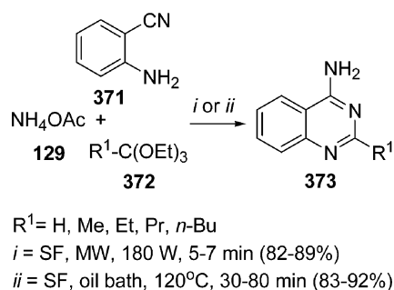
Scheme 111
