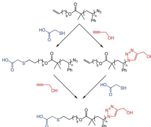
Scheme 11 \alpha,\omega -Functional polystyrene via sequential thiol-ene/alkyne-azide couplings, or vice versa .
