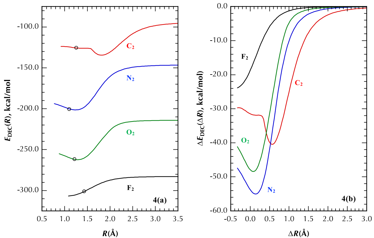
Fig. 4. (a) The total dynamical electron correlation energy, E_{\text{DEC}}(R) , for the ground states of \text{C}_2 , \text{N}_2 , \text{O}_2 and \text{F}_2 , and (b) the dynamical electron correlation energy relative to that of the separated atoms ( R = 20.0 Å) shifted by the calculated equilibrium internuclear distances, \Delta E_{\text{DEC}}(\Delta R) , where \Delta R = R - R_e . In Fig. 4(a) the circles on each curve are located at the calculated R_e for the given molecule. The minima in the \Delta E_{\text{DEC}}(\Delta R) curves in (b) are at \Delta R = 0.57 Å ( \text{C}_2 ), 0.14 Å ( \text{N}_2 ) and 0.08 Å ( \text{O}_2 ).
