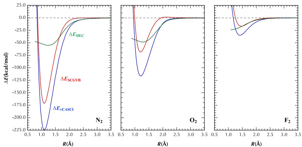
Fig. 6 Potential energy curves, \Delta E_{\text{SCGVB}} and \Delta E_{\text{vCASCI}} , for the ground states of \text{N}_2 , \text{O}_2 and \text{F}_2 along with the changes in the dynamical correlation energies relative to that of the separated atoms, \Delta E_{\text{DEC}}(R) .
