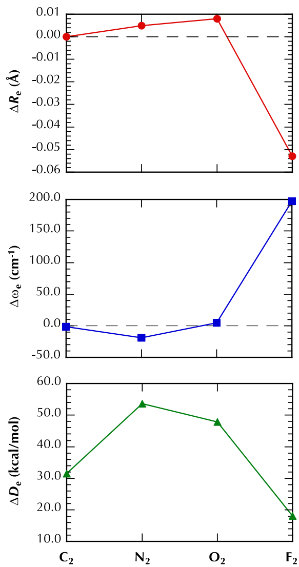
Fig. 1 Changes in the spectroscopic constants of C 2 –F 2 resulting from inclusion of dynamical electron correlation, e.g., \Delta R_e = R_e(\nu\text{CASCI}) - R_e(\text{SCGVVB}) .
