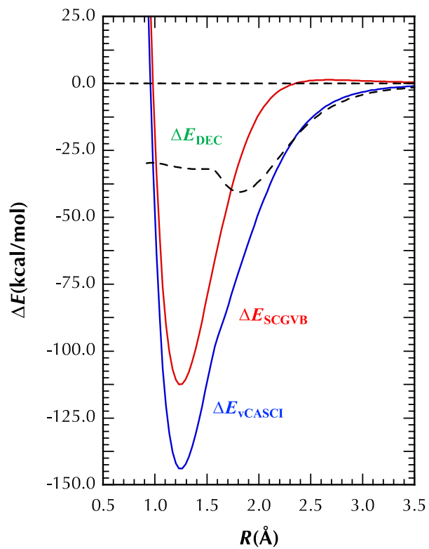
Fig. 3 The potential energy curves, \Delta E_{\text{SCGVB}} and \Delta E_{\text{vCASCI}} , for the X^1\Sigma_g^+ state of \text{C}_2 along with \Delta E_{\text{DEC}}(R) . The minima in the potential energy curves are at R_e = 1.244 \text{ \AA} (SCGVB) and 1.248 \text{ \AA} (vCASCI). The minimum in the \Delta E_{\text{DEC}}(R) curve is at 1.82 \text{ \AA} . The visible bend in \Delta E_{\text{vCASCI}} at R = 1.59 \text{ \AA} is due to the interaction between the X^1\Sigma_g^+ and B^1\Sigma_g^+ states.
