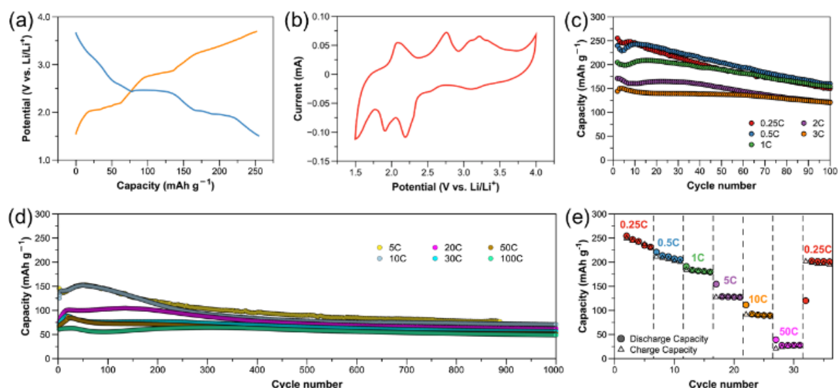
Fig. 2 Electrochemical properties of [CuL(Py) 2 ] n cathode: (a) Discharge-charge profile at 0.25C (~65 mA g -1 ). (b) CV plot with a scan rate of 0.5 mV s -1 . (c) Capacity retention at rates of 0.25C to 3C (~785 mA g -1 ). (d) Capacity retention at rates of 5C (~1308 mA g -1 ) to 100C (~26162 mA g -1 ). (e) Rate capability at various current densities.
