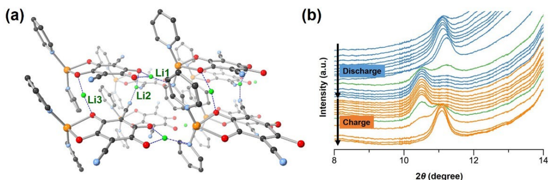
Fig. 5 (a) Computational simulation of lithiated CP [\text{CuL}(\text{Py})_2\text{Li}_3]_n showing the DFT optimized structure. Colours of atoms: orange: Cu(I); grey: C; red: O; cyan: N; green: Li; H is omitted for clarity. (b) In situ synchrotron PXRD patterns of CP electrode collected during the first discharge-charge cycle at current density of 120 \text{ mA g}^{-1} at a voltage between 1.5 V and 4.0 V.
