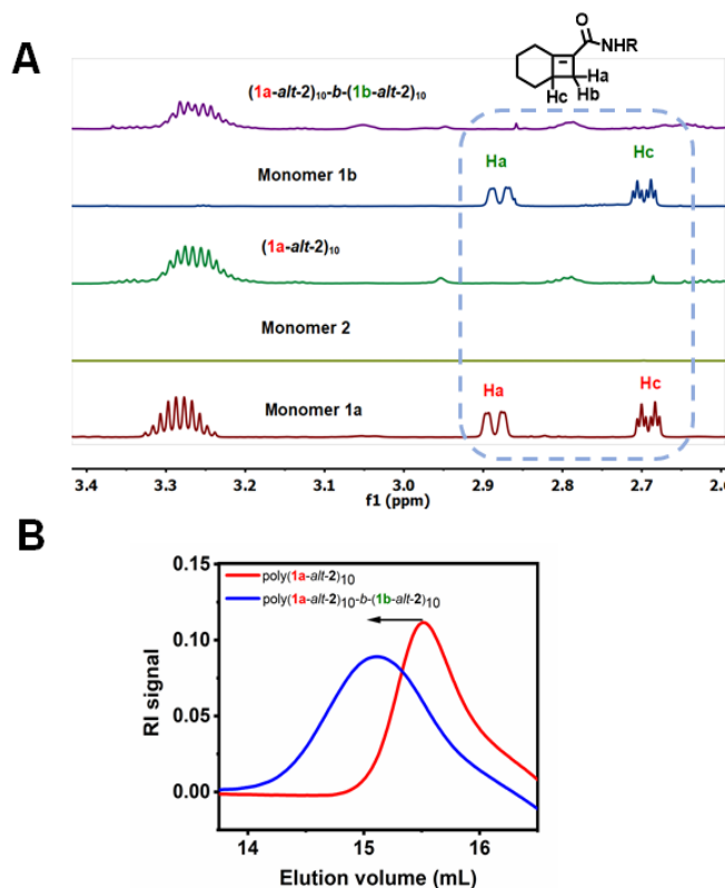
Fig. 3 Diblock copolymer P3 was successfully prepared in two steps. In step 1, monomer 1a was fully incorporated to form the first block, and monomer 1b was fully incorporated at step 2 to install the second block as shown by both the 1 H-NMR overlay (A) and GPC chromatogram (B).
