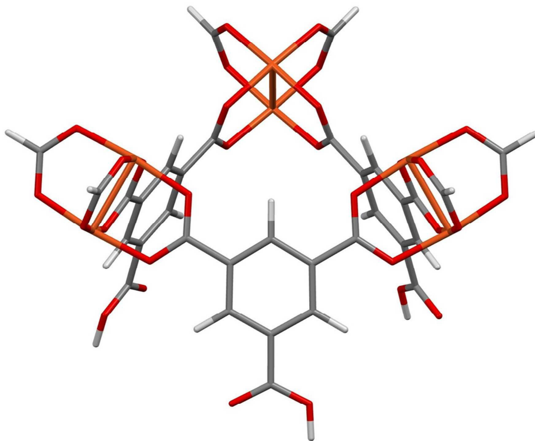
Figure 3: The small fragment chosen to model the small pore in HKUST-1. Adapted from CSD Refcode DOTSOV.
