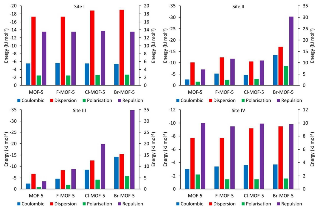
Figure 10: PIXEL component energies for the four H 2 adsorption sites in MOF-5 and its halogen functionalised analogues. Repulsion bars correspond to the right hand axis, others to the left axis.
