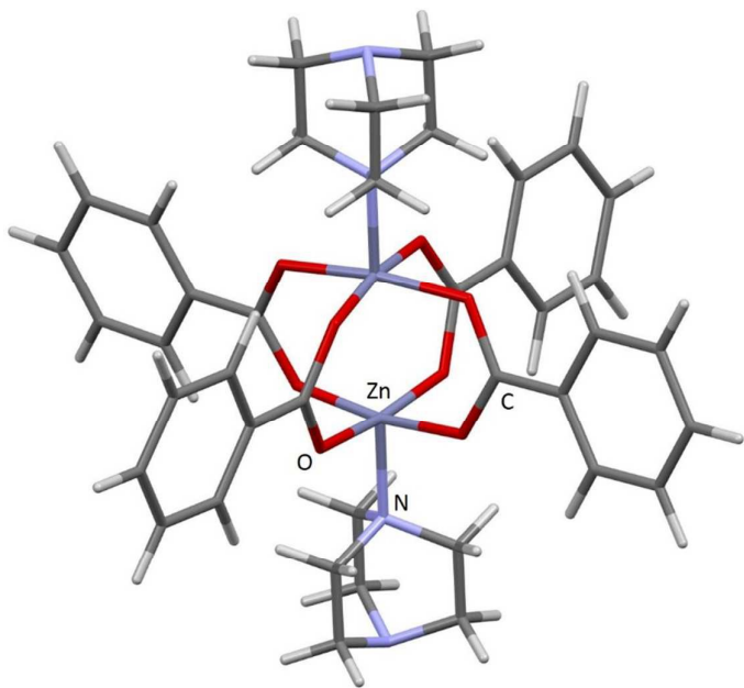
Figure 2: The fragment model of Zn 2 (BDC) 2 (TED). Adapted from CSD Refcode HEGKAP.
