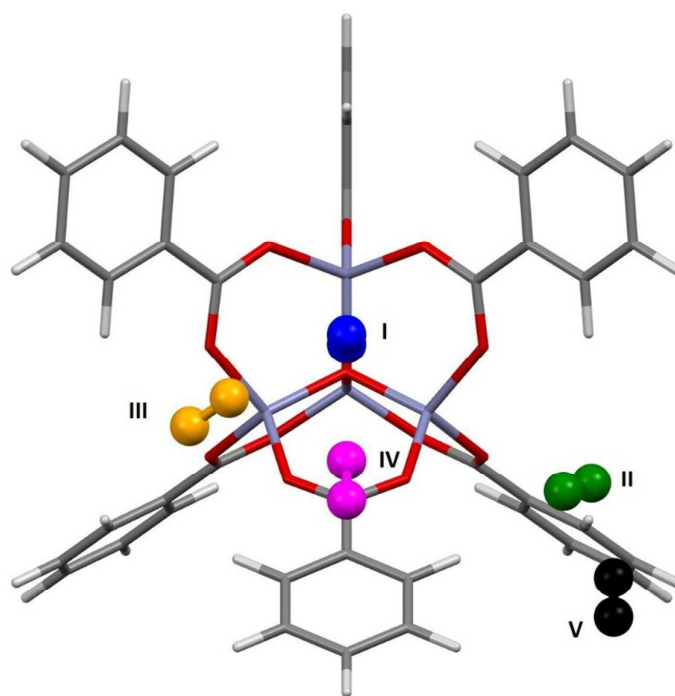
Figure 5: N 2 adsorption sites in MOF-5 located using PIXEL.
