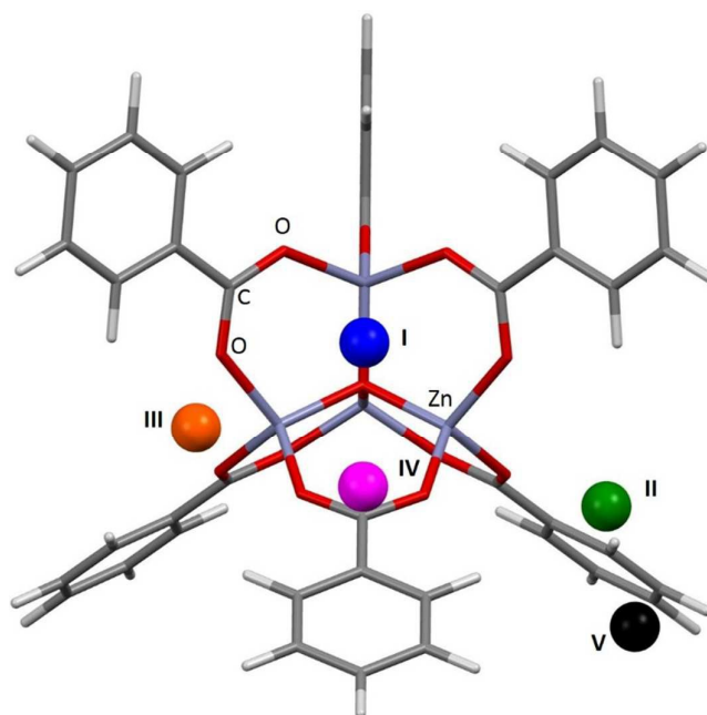
Figure 1: The five adsorption sites associated with the framework structure of MOF-5. The locations of these sites were obtained from single crystal diffraction data (CSD Refcode LAWFUL). 17
