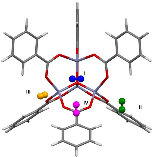
Figure 6: The most favourable orientations of the H 2 molecules found using PIXEL at sites I-IV in MOF-5.
