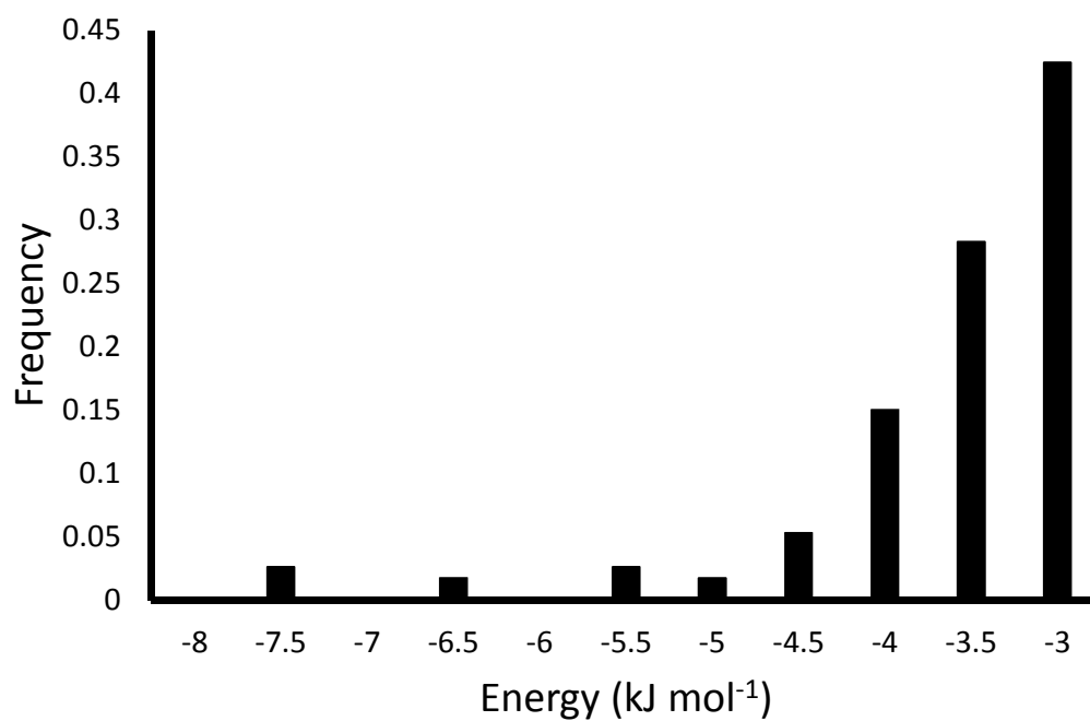
Figure 8: Energy frequency for the first 100 binding sites of H 2 in Zn 2 (BDC) 2 (TED) as calculated by PIXEL.
