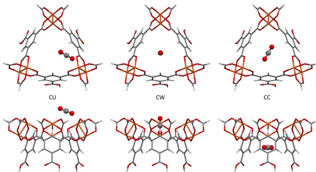
Figure 9: The three independent CO 2 adsorption sites found in HKUST-1 viewed perpendicular (top) and parallel (bottom) to the small cage opening.
