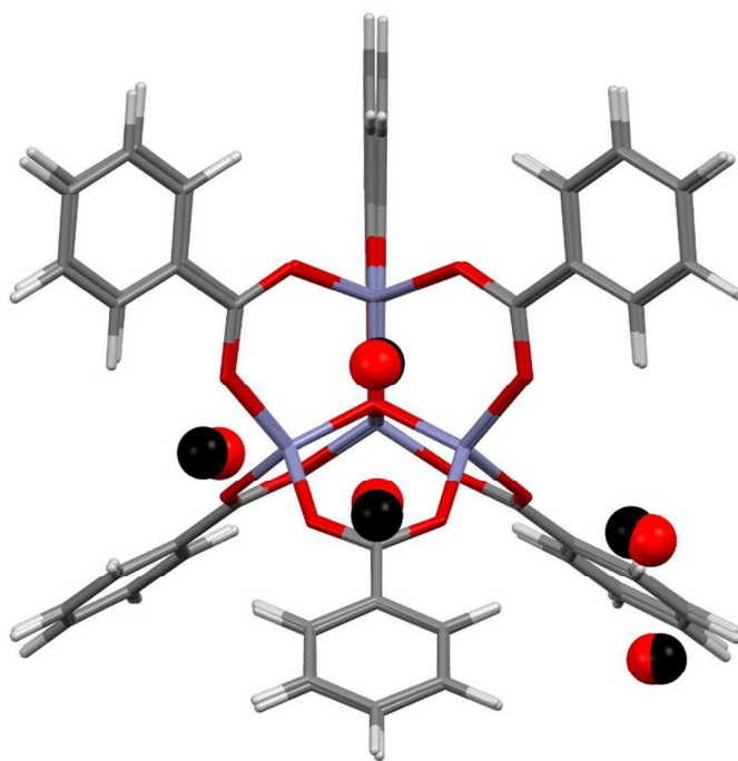
Figure 4: Overlay of Ar adsorption sites in MOF-5 located using PIXEL (red) with those obtained experimentally (black). Adapted from CSD Refcode LAWFUL.
