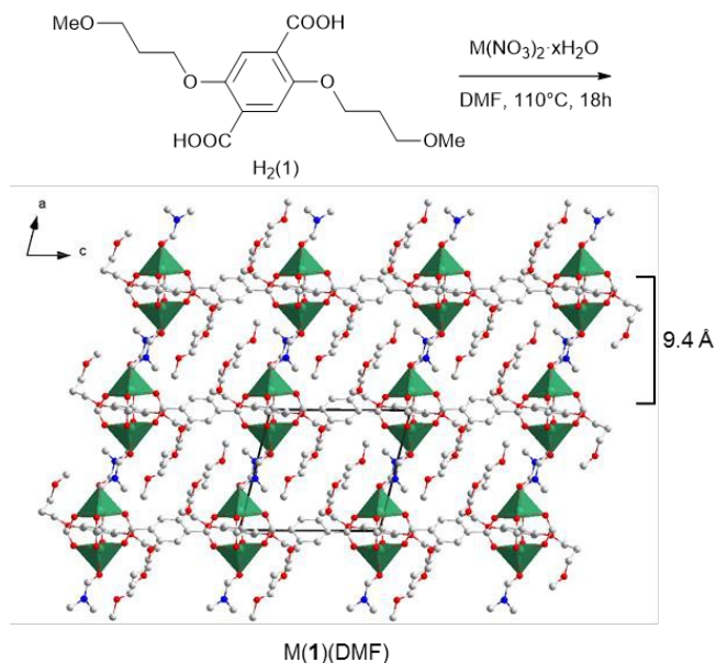
Fig. 1: Reaction scheme for the synthesis of M(1)(DMF) (with M = Cu, Zn ) showing crystal structure of Zn(1)(DMF) viewed along the b -axis highlighting the lamellar structure with an interlayer spacing of \sim 9.4 \text{ \AA} ( \sim 9.6 \text{ \AA} for Cu(1)(DMF) ). C, N and O atoms are shown in grey, blue and red. The coordination polyhedra of the M ions are displayed in green. H atoms have been omitted for clarity.
