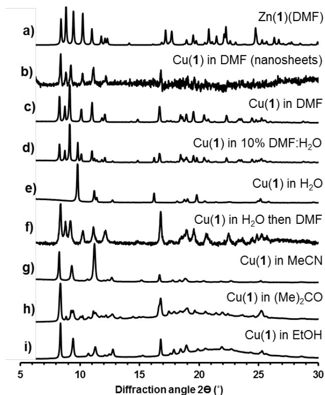
Fig. 3: a) Calculated XRPD pattern for Zn(1)(DMF). Experimental XRPD patterns for b) nanosheets of Cu(1) exfoliated in DMF ** , solids collected following exfoliation of Cu(1)(DMF) in c) DMF, d) 10% DMF-water, e) water, f) water, followed by reimmersion in DMF for 4 days ** , g) acetonitrile, h) acetone * , and i) ethanol * . Patterns marked with an * were measured using Kapton capillaries to prevent solvent loss, those with a # are background subtracted patterns, other measurements were collected using dried powders on flat substrates.
