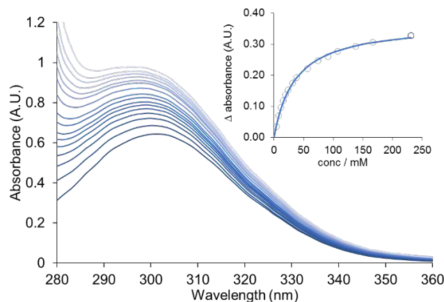
Fig. 4: UV-vis titration showing addition of aliquots of a pyridine solution to an aqueous suspension of Cu(1) nanosheets. Insert shows a plot of change in absorbance against concentration of pyridine which is fitted to calculate the binding constant for pyridine to the nanosheets ( K_a = 30 \pm 8 \text{ M}^{-1} ).
