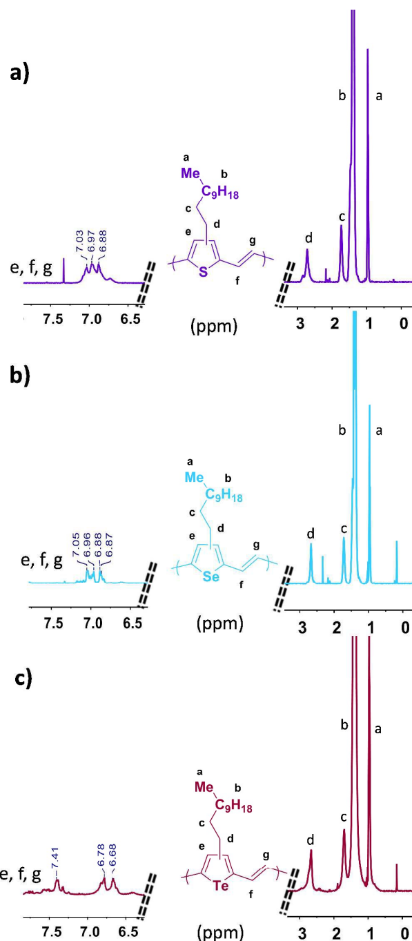
Figure 1. ^1\text{H} NMR spectra of the three polymers; (a) P3TV , (b) P3SV and (c) P3TeV (500 MHz, \text{C}_2\text{D}_2\text{Cl}_4 , 130 °C).
