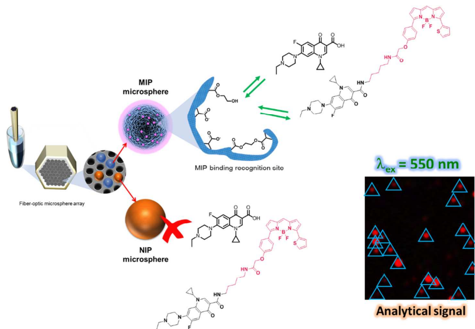
Fig. 2. Workflow of the assay protocol. ENRO quantification was based on a competitive assay in which the target analyte competes with the labeled ENRO (BODIFLOXACIN) to bind to specific binding sites on the MIP microspheres.
