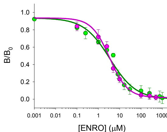
Fig. 8 Comparison of competitive calibration curves in 50:50 (v/v) MeCN:HEPES (25 mM pH 7.5) (green points, n = 4 , 14 points) and in serum (with dilution of 1/6, pink points, n = 3 , 9 points). It is plotted B/B_0 versus different concentrations of ENRO, which competes with BODIFLOXACIN.
