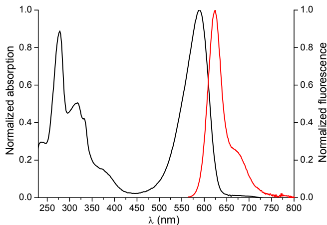
Fig. 4 Normalized absorption (black) and emission (red) spectra of BODIFLOXACIN in MeCN (3.57 \mu\text{M} ) upon excitation at 560 nm. The absorption and emission maxima were \lambda_{abs}^{max} = 588 \text{ nm} and \lambda_{em}^{max} = 624 \text{ nm} , respectively.
