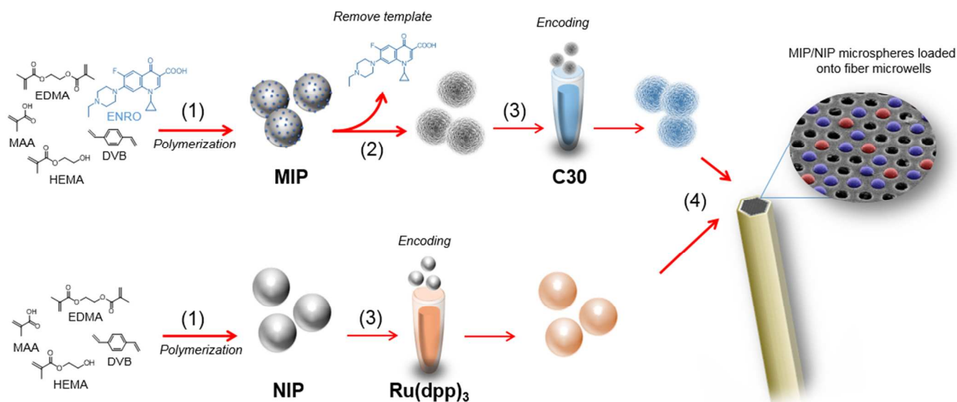
Fig. 1. Workflow of the microarray fabrication. (1) MIP microspheres selective to ENRO and NIP microspheres used as control, were prepared following a precipitation-polymerization approach. (2) MIP microspheres were extensively washed with MeOH:TFA (95/5, v/v), MeOH, followed by acetone until no trace of the template was observed. (3) MIP and NIP microspheres were then encoded with C30 and [Ru(dip) 3 ]Cl 2 in THF and THF:MeCN (70:30, v/v), respectively. (4) A suspension of 0.25 mg mL -1 of NIP and MIP microspheres were prepared in MeCN, and a drop of 1 \mu L of the suspension was deposited onto the etched distal end of the fiber.
