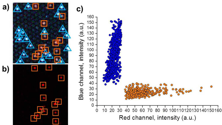
Fig. 3. Micrographs that show a) fluorescence of coumarin-30 and [Ru(dip) 3 ]Cl 2 exciting at 405 nm, and b) fluorescence of [Ru(dip) 3 ]Cl 2 exciting at 470 nm. c) Population distribution intensities of red and blue channels of MIP (encoded with coumarin-30, blue points, n = 734) and NIP (encoded with [Ru(dip) 3 ]Cl 2 , orange points, n = 382) microspheres.
