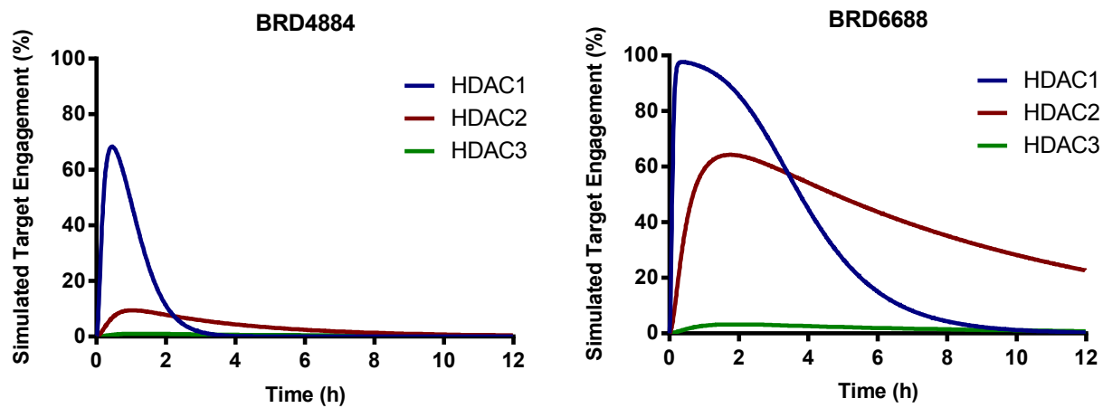
Figure 2. Simulated target engagement profiles for HDAC 1, 2 and 3 in brain for BRD4884 and BRD6688 at 10 mg/kg dose.
