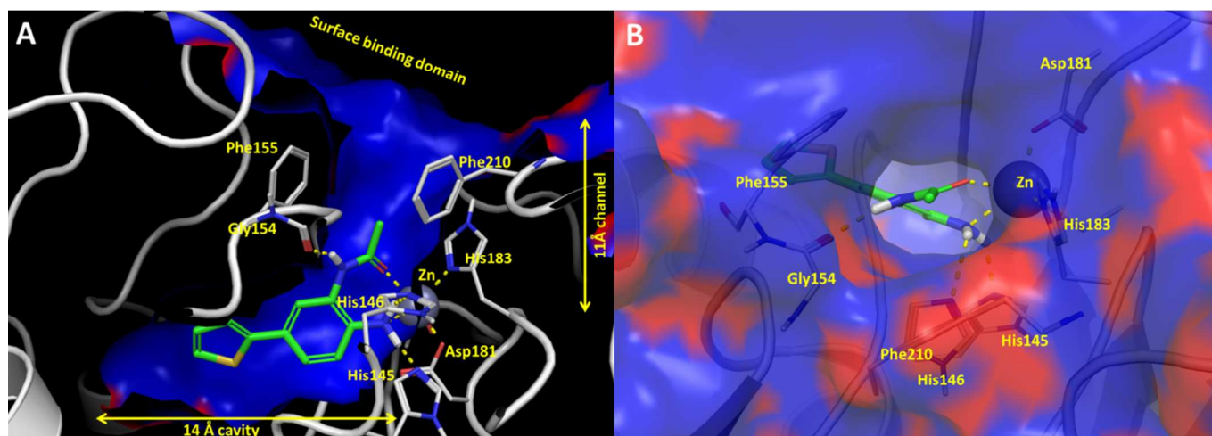
Figure 1. A) Cross sectional view of compound 3 docked into catalytic binding domain of HDAC2 B) Solvent view of compound 3 docked into HDAC2 showing the trajectory of the sp^3 methyl amide into the 11Å channel. Hydrogen bonding interactions are shown as yellow dotted lines. The electrostatic surface of HDAC2: blue = hydrophobic regions; red = negatively charged regions.
