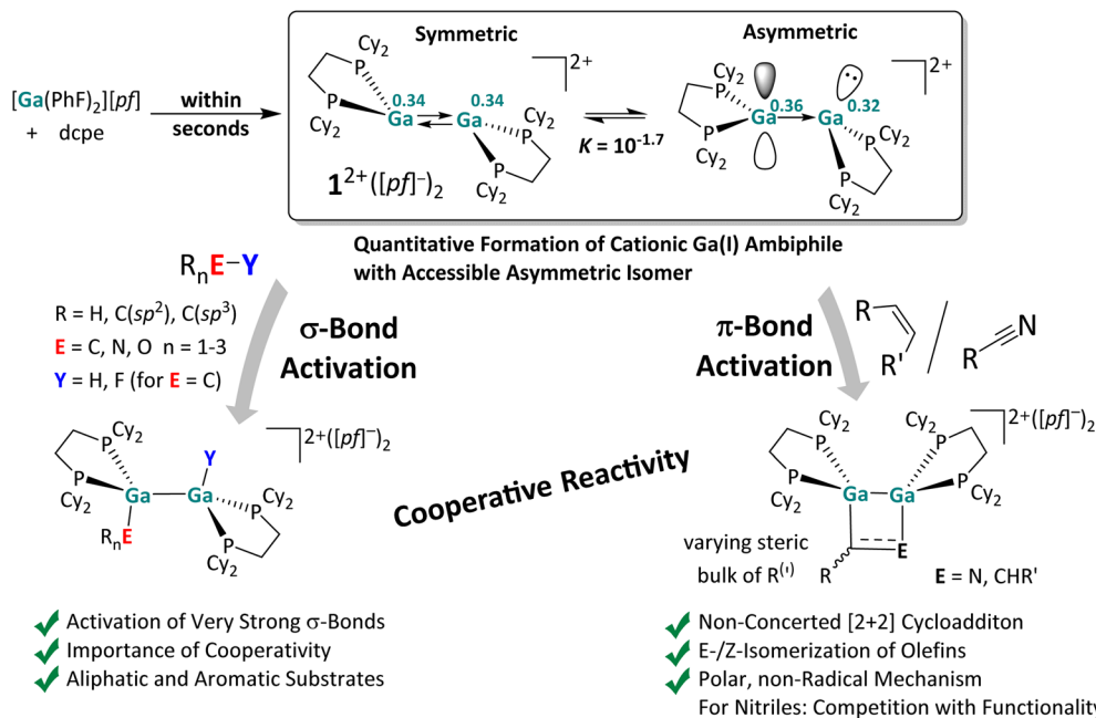
Scheme 10 Results of this work. The in situ formed reactive digallene 1^{2+} accessible from [Ga(PhF)_2][pfl] and commercial dcpe , 29 reacts cooperatively and with strong contributions from the accessible asymmetric conformer (QTAIM charges on Ga atoms are written in superscript) with olefins, nitriles and strong C–F, C–H, N–H, and O–H \sigma -bonds. The herein derived mechanistic insight will help to pick up selected activations and to transform them into parts of catalytic cycles, especially in those cases, where the energetics underlying the activations is only moderately exergonic or even on the edge (olefins, N–H, O–H, and CN-cycloaddition).
