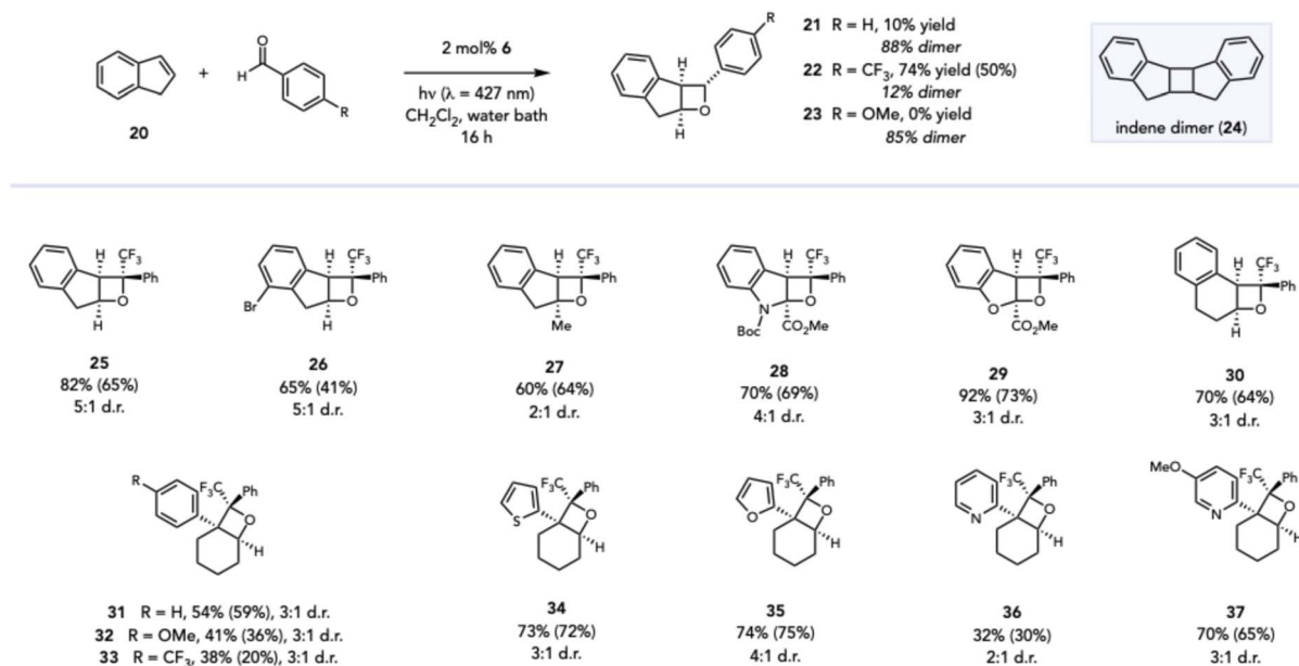
Fig. 4 Scope studies for transposed Paternò–Büchi reactions of indenes and arylcyclohexenes. Assay yields and d.r. determined by crude 1 H NMR analysis using CH 2 Br 2 as an internal standard. Isolated yields of the combined diastereomers reported in parentheses.
