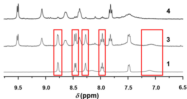
Fig. 2 ^1\text{H} NMR spectra of 1 , 3 and 4 (300 MHz, \text{d}_6\text{-DMSO} , 298 K). For clarity, only the aromatic region is shown here.
