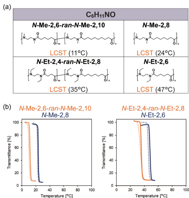
Fig. 5 (a) Chemical structure of random copolymers adjusted their hydrophilic/hydrophobic balance to C 6 H 11 NO and N-alkylated nylon homopolymers with C 6 H 11 NO. (b) Transmittance change at 800 nm of N-alkylated nylon random copolymers (orange) and homopolymers (blue) in H 2 O (10 mg mL -1 ) by the temperature changes (scan rate: 1.5 °C min -1 ); the solid and dotted lines represent the heating and cooling processes, respectively.
