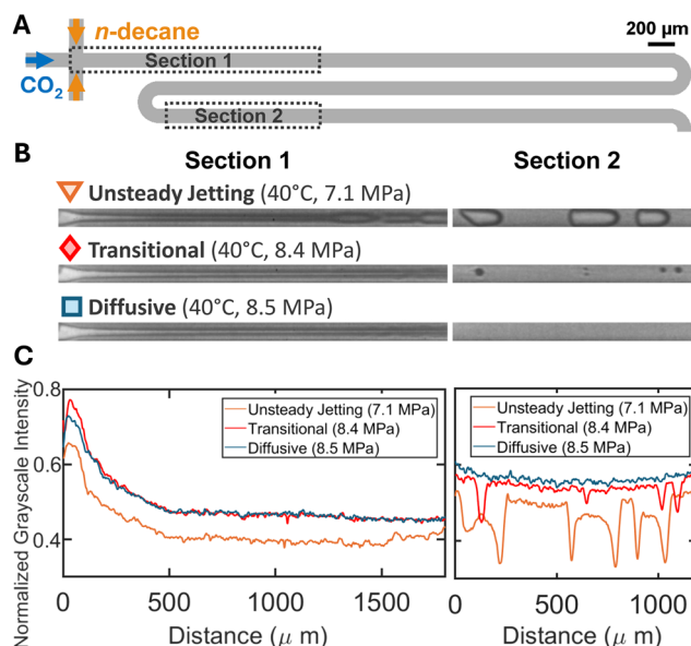
Fig. 13 (A) Microchannel schematic indicating section 1 and section 2 as the defined regions of interest (ROI). Section 1 is positioned at the junction where the CO_2 -decane interface forms, while section 2 is located 8.6 mm downstream. Scale bars: 200 \mu m . (B) Experimental snapshots at section 1 (left) and section 2 (right) for unsteady jetting (40 °C, 7.1 MPa), transitional (40 °C, 8.4 MPa), and diffusive (40 °C, 8.5 MPa) regimes. (C) Grayscale intensity profiles (normalized to 0–1) along the flow direction for each ROI, averaged across the channel width from the corresponding snapshots in (B).
