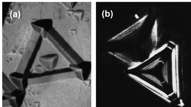
Fig. 8 (a) Triangular etch pits in 3C-SiC. Reproduced with permission. 85 Copyright 1997, Wiley-VCH. (b) Distorted hexagonal etch pits in the 4H and 6H-SiC. Reproduced with permission. 86 Copyright 2005, Elsevier.
