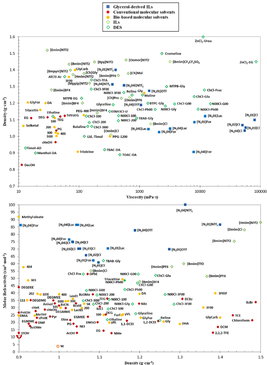
Fig. 11 Properties maps of developed glycerol-derived ILs [N 2 O R ]X (in blue) with respect to common ILs and DES (in green), traditional molecular solvents (in red) and bio-based molecular solvents (in gold), representing density vs. viscosity and molar refractivity vs. density.
