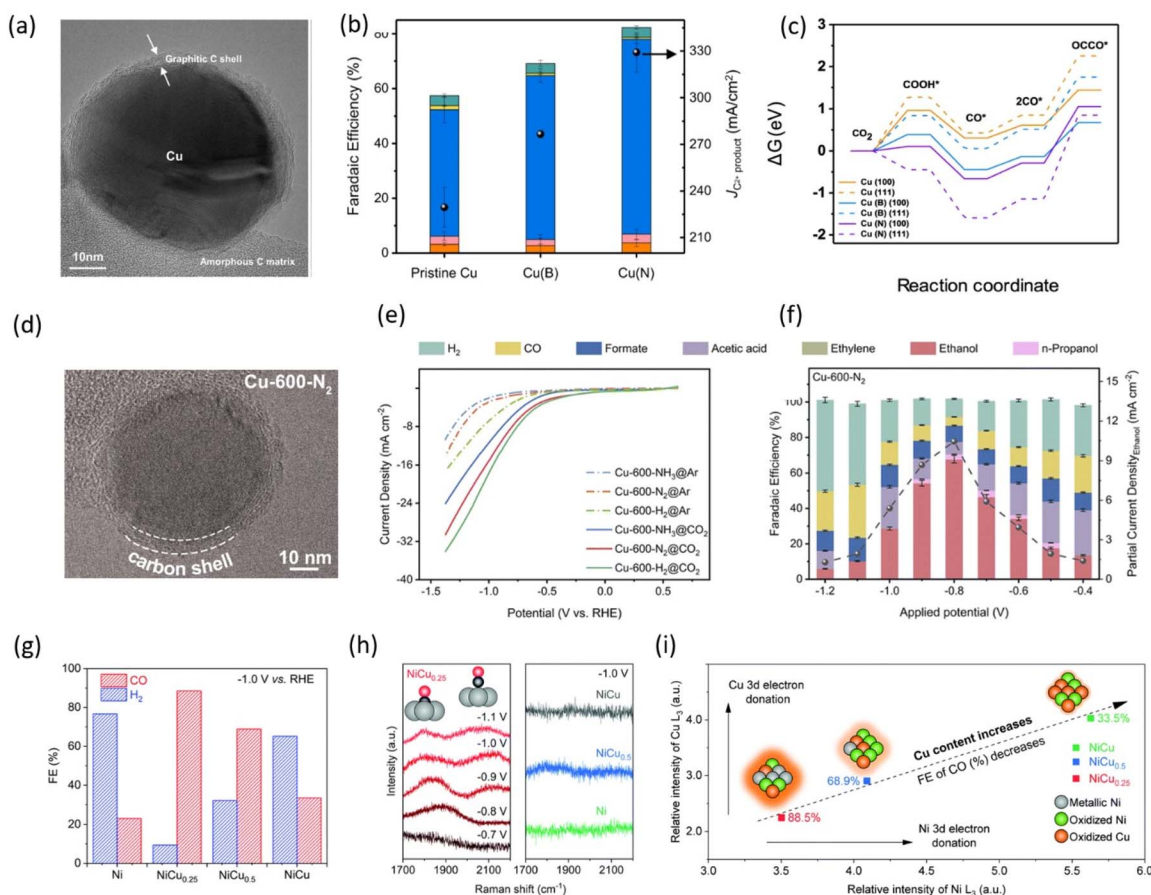
Fig. 13 Graphene-shell encapsulated metal nanoparticles for \text{eCO}_2\text{RR} (a) high-resolution TEM image of the confined Cu nanoparticles and quasi-graphitic C shell. (b) FE and partial current density for \text{C}_{2+} products at 400 mA cm -2 . (c) Free energy diagram for CO dimerization on the pristine Cu, Cu (B), and Cu (N) surfaces. Adapted with permission from ref. 68 Copyright 2021, Springer Nature. (d) TEM images of Cu-600-N 2 . (e) LSV curves in \text{CO}_2 and Ar-saturated 0.1 M \text{KHCO}_3 aqueous solutions for Cu-600-N 2 , Cu-600-H 2 , and Cu-600-NH 3 . (f) FE and partial current density for Cu-600-N 2 . Adapted with permission from ref. 127 Copyright 2023, Royal Society of Chemistry. (g) FE distributions at 1.0 V vs. RHE. (h) In situ Raman spectroscopy results. Left: Potential-dependent Raman spectra of \text{NiCu}_{0.25} , with adsorption models illustrating ^*\text{CO} adsorption at bridge and atop sites on the catalyst surface. Right: Raman spectra of other catalysts recorded at an applied potential of 1.0 V vs. RHE. (i) Electron donation and CO selectivity trend with increasing Cu content in \text{NiCu}_x . Glow intensity represents 3d electron density in molecular models. Adapted with permission from ref. 128 Copyright 2017, Royal Society of Chemistry.
