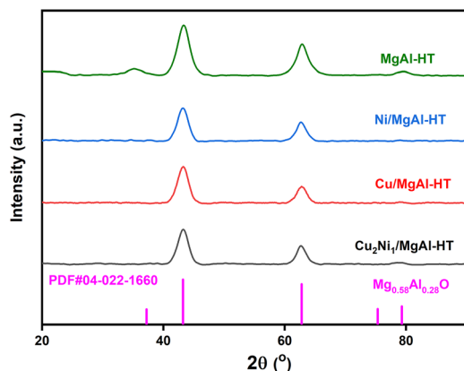
Fig. 3 XRD patterns of the MgAl-HT, Ni/MgAl-HT, Cu/MgAl-HT and \text{Cu}_2\text{Ni}_1/\text{MgAl-HT} catalysts.
