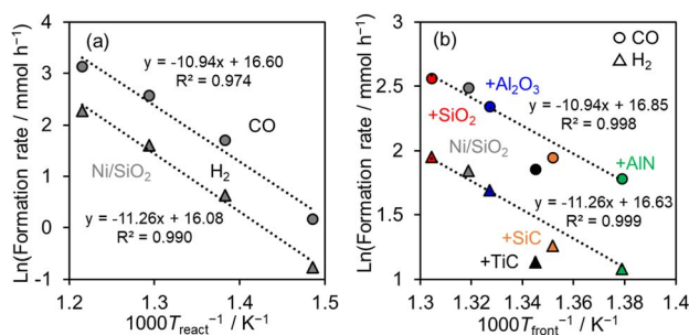
Fig. 5 (a) Arrhenius plot of the Ni/SiO 2 catalyst and (b) relationship between photothermal catalytic activities and T_{\text{front}} values of the mixed catalysts.
