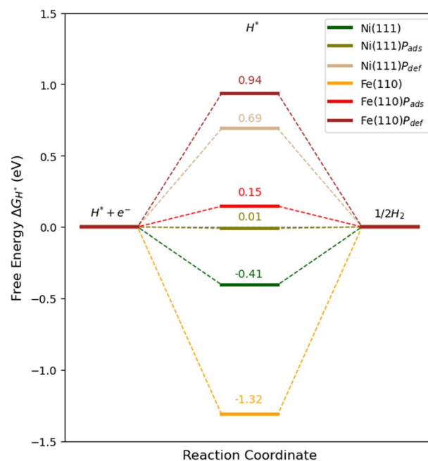
Fig. 8 Gibbs free energy diagram ( \Delta G_{H^*} ) for hydrogen adsorption on various Ni(111) and Fe(110) surfaces, including pristine, adsorbed P ( P_{ads} ), and P adsorbed in defect ( P_{def} ) configurations.
