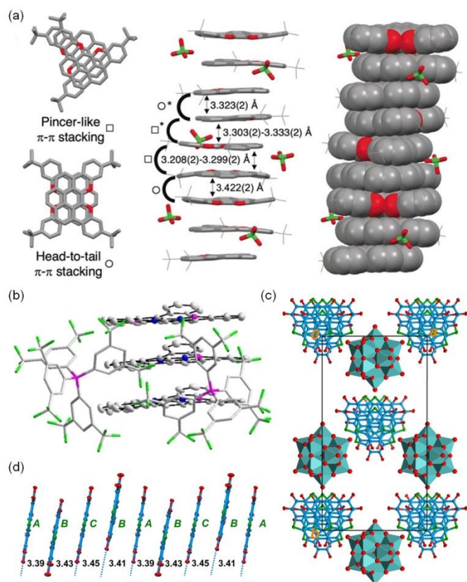
Fig. 20 (a) \pi - \pi stacking in the crystal structure of 60b 3 (ClO 4 ) 2 ·THF·(H 2 O) 0.5 ; (b) \pi -stacked trimer in the crystal structure of 61b 3 2+ [(BAR F 4 ) - ] 3 ; (c) a unit cell in the crystal structure of 62a 4 3+ (PMo 12 O 40 ) 3- ; (d) \pi - \pi stacking in the crystal structure of 62a 4 3+ (PMo 12 O 40 ) 3- . Reproduced with permission from ref. 110–112. Copyright 2020, 2023 and 2024 Wiley.
