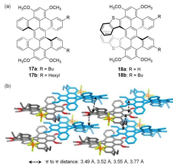
Fig. 6 (a) Double helixenes 17a/b and 18a/b ; (b) \pi - \pi stacking in the crystal of 17a •+ PF 6 − , where the (M, M) enantiomer is shown in blue, and the (P, P) enantiomer is colored according to the elements. Reproduced with permission from ref. 40. Copyright 2022 American Chemical Society.
