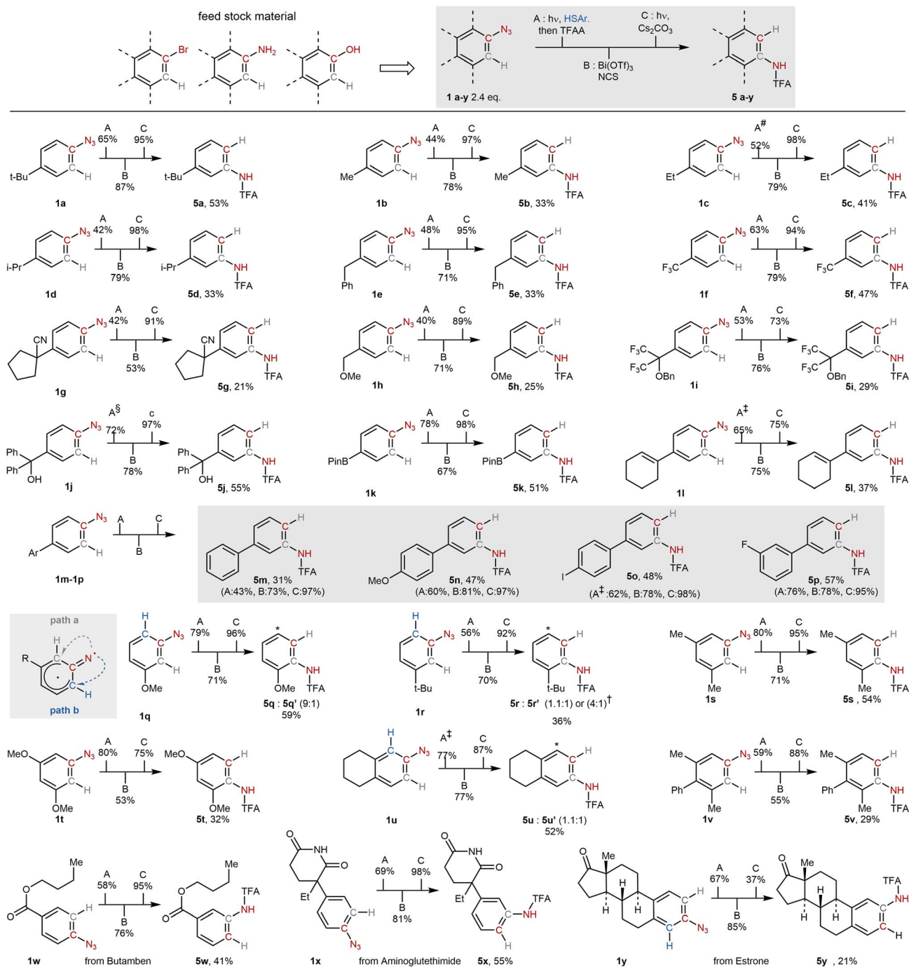
Scheme 4 Substrate scope of the nitrogen regioisomerization. Solvent: # hexane, § diethyl ether, ‡ trifluorotoluene, † step A: trifluorotoluene 60 °C. Conditions: A: DMAP (1 eq.), 1,4-dioxane (0.05 M), hv = 390 nm, r.t., 16 h, then TFAA (4 eq.), r.t., 2h. B: NCS (1 eq.), Bi(OTf) 3 (1 eq.), 1 : 1 1,4-dioxane/MeCN (0.033 M), r.t., 6 h. C: Cs 2 CO 3 (1 eq.), 1 : 1 MeOH/Acetone (0.05 M), hv = 390 nm, r.t., 12 h. Yield : A = yield calculated based on the amount of thiol used, A and B = NMR yield, C = isolated yield.
