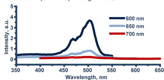
Fig. 4 Photophysical properties studies of 3. (A) Absorption spectra in acetonitrile as a function of percentage of water, 25 °C. (B) Emission spectra in PBS as a function of molarity of solution, RT. (C) Excitation spectra as a function of emission wavelength in PBS, RT (derived from Fig. S68–70†).
