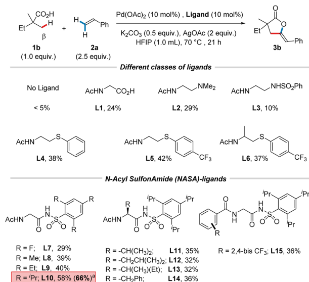
Scheme 2 Optimization of the reaction conditions. Reactions were conducted on a 0.1 mmol scale. Yields were determined by ^1\text{H} NMR analysis of the crude reaction mixture using \text{CH}_2\text{Br}_2 as an internal standard. * \text{MnO}_2 (20 mol%) was added.
