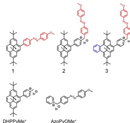
Fig. 3 Studied derivatives.
