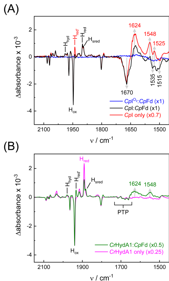
Fig. 5 Infrared difference spectroscopy. (A) \text{H}_2 - \text{N}_2 ATR FTIR difference spectra of Y3pCNF- CpFd : CpI (black) and CpI alone (red) after 25 s. Bands above 1750\text{ cm}^{-1} are assigned to H-cluster ligands in the H_{\text{ox}} state (negative) and various reduced states (positive). At lower frequencies, the 1670/1624\text{ cm}^{-1} down-shift in the amide I regime indicates protein structural changes, alongside up-shifts at 1535/1548\text{ cm}^{-1} and 1515/1525\text{ cm}^{-1} . The blue spectrum serves as a negative reference where CpI was inactivated with \text{O}_2 ahead of the reaction with \text{H}_2 . (B) \text{H}_2 - \text{N}_2 ATR FTIR difference spectra of Y3pCNF- CpFd : CrHydA1 (green) and CrHydA1 alone (magenta) after 50 s. Note the lack of the difference features in CrHydA1 in the amide I regime while only small changes are observed in the presence of Y3pCNF- CpFd . "PTP" refers to small difference features explored earlier. 62 All spectra are normalized to the main CO band of H_{\text{ox}} ( 1947\text{ cm}^{-1} in CpI , 1940\text{ cm}^{-1} in CrHydA1 ) with factors as indicated in the legends.
