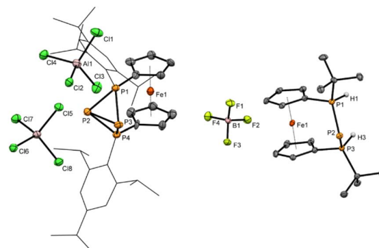
Fig. 2 Molecular structures of 4[\text{AlCl}_4]_2 and 8c[\text{BF}_4] in the solid state. Ellipsoids are shown at 30% probability. All hydrogen atoms except H1 and H3, which are bonded to phosphorus atoms are omitted for clarity. The Tip substituents at P1 and P4 in 4[\text{AlCl}_4]_2 are shown as wireframe. Selected bond lengths and angles in 4[\text{AlCl}_4]_2 : P1–P2 2.184(5) Å, P1–P3 2.171(5) Å, P2–P3 2.335(5) Å, P2–P4 2.194(5) Å, P3–P4 2.173(5) Å; 8c[\text{BF}_4] : P1–P2 2.1284(7) Å, P2–P3 2.1265(7) Å, P1–H1 1.28(2) Å, P2–H2 1.26(2) Å, PPP-angle 89.50(2)^\circ .
