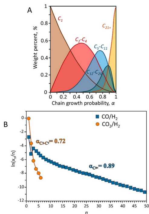
Fig. 3 (A) Hydrocarbon distribution predicted by ASF model. Adapted from ref. 53 and (B) hydrocarbons experimental ASF plots reported in terms of selectivity during CO and \text{CO}_2 hydrogenation. Adapted from ref. 54.
