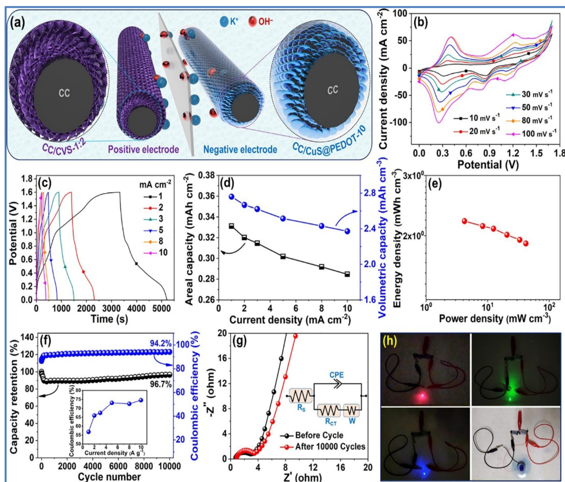
Fig. 14 (a) Schematic of \text{CC/CVS-1:2} // \text{CC/CuS@PEDOT-10} asymmetric device, electrochemical properties of \text{CC/CVS-1:2} // \text{CC/CuS@PEDOT-10} asymmetric device (b) CV at various \nu (c) GCD at various I_d (d) areal capacity vs. I_d (e) Ragone plot (f) capacity retention and \eta over 10 000 cycles (g) EIS plot before and after cycling with fitted equivalent circuit, and (h) illuminating red, green, and blue LEDs and powering a small electrical motor fan using two serially connected \text{CC/CVS-1:2} // \text{CC/CuS@PEDOT-10} asymmetric device (reproduced from ref. 45 with permission from Elsevier© 2022).
