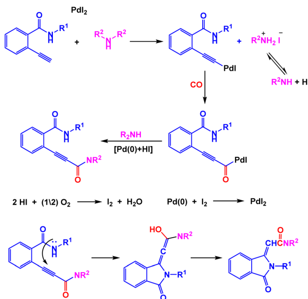
Scheme 15 Rational pathway for synthesis of 3-[(dialkylcarbamoyl)methylene]isindolin-1-ones through \text{Pd}_2 -catalyzed oxidative carbonylation conditions.
