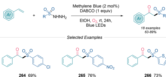
Scheme 28 Photoredox \beta -ketosulfone synthesis described by Zhu. 51
