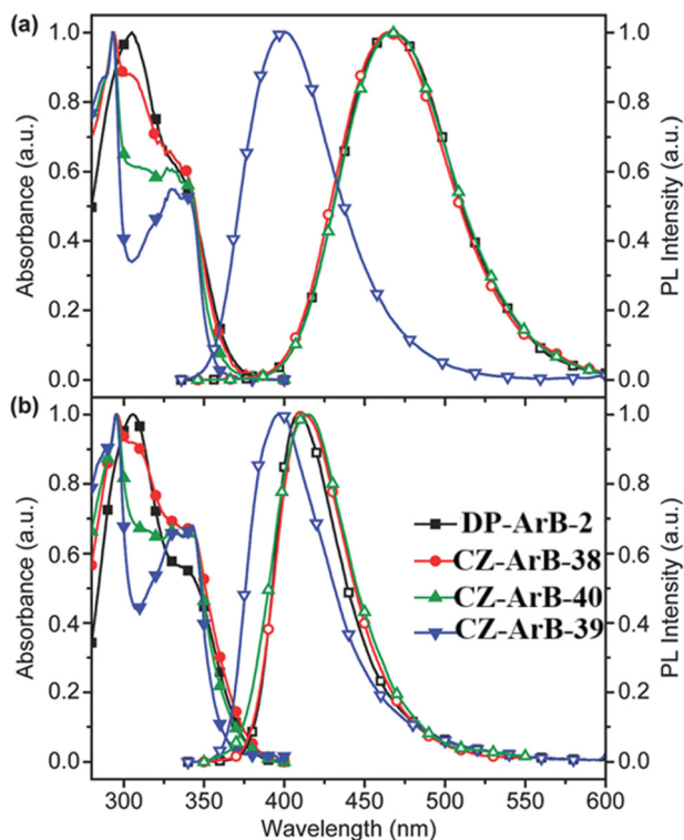
Fig. 20 UV-absorption (solid symbols) and emission spectra (open symbols) of DP-ArB-2 , CZ-ArB-38–40 in (a) DCM solution and (b) solid films. Reproduced with permission from ref. 126. Copyright 2018 Wiley.
