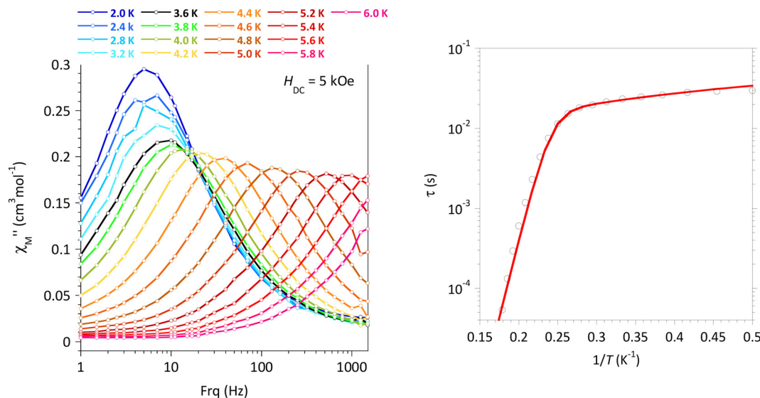
Fig. 3 [FeL NS Br 2 ], 3 : (left panel) \chi'' versus \nu , in the 2–6 K temperature range with H_{DC} = 5 kOe; (right panel) experimental (O) and calculated (—) relaxation time, \tau , versus 1/T with best-fit associated with eqn (6) (see the main text).
