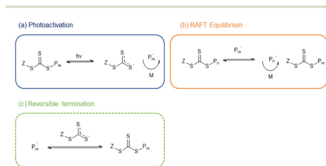
Scheme 1 General mechanism of PI-RAFT polymerisation. The S–C bond is photolysed to generate a free radical (a, photoactivation). The propagating radical can either chain transfer the active centre (b, RAFT equilibrium) or combine with a photoiniferter radical to terminate reversibly (c, reversible termination).
