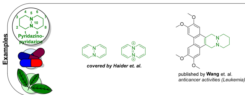
Fig. 7 Examples of pyridazino-pyridazine-derived compounds.
