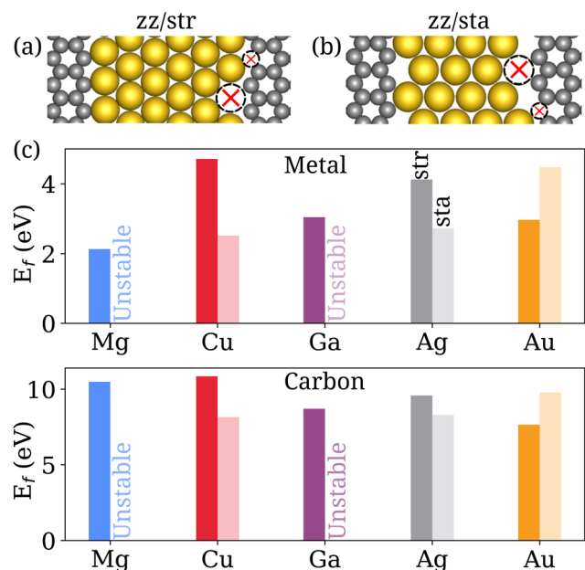
Fig. 7 Atom vacancy models for the interfaces. Vacancies (a) at zz/str and (b) zz/sta interfaces. The vacancy candidates were selected based on our charge transfer analysis and marked with red crosses. (c) The formation energies of a metal/carbon defects at the interface. Staggered edges are indicated by a brighter color and straight edges by a darker one.
