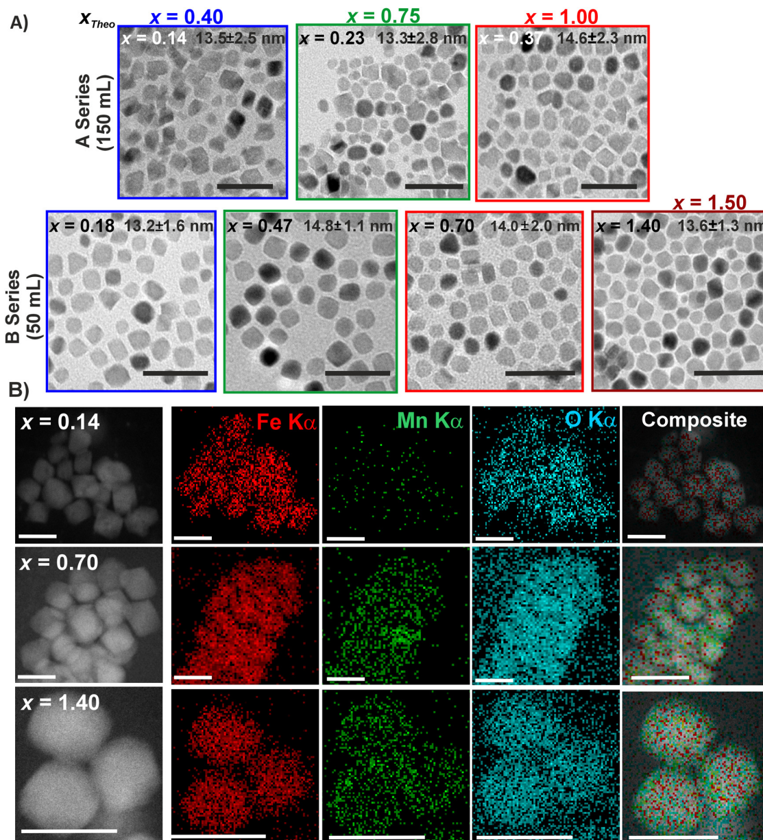
Fig. 1 (A) TEM images of Mn x Fe 3-x O 4 MNPs with varying Mn 2+ content ( x_{Empiric} = 0.14 to 1.40 ). The samples with the initial Fe/Mn precursor amount of x_{Theo} = 0.40, 0.75, 1.0 , and 1.50 are highlighted with blue, green, red, and brown boxes, respectively. Inset: Empirical x value for each sample determined by ICP-OES along with their respective size diameters. Scale bar: 50 nm. (B) STEM-EDX mapping images of Mn x Fe 3-x O 4 MNPs with the lowest, medium, and highest content of Mn 2+ ( x_{Empiric} = 0.14, 0.70, 1.40 ). Scale bar: 50 nm ( x_{Empiric} = 0.14 and 0.70 ), 20 nm ( x_{Empiric} = 1.40 ).
