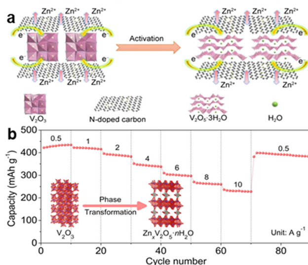
Fig. 5 Schematic of (a) Chemical conversion mechanism of \text{V}_2\text{O}_3 . 16 Copyright 2023, Springer Nature Limited. (b) Phase transition from \text{V}_2\text{O}_3 to \text{Zn}_{0.4}\text{V}_2\text{O}_5 \cdot n\text{H}_2\text{O} in static Zn–V batteries (vanadium-based zinc-ion batteries). 13 Copyright 2021, Elsevier.
