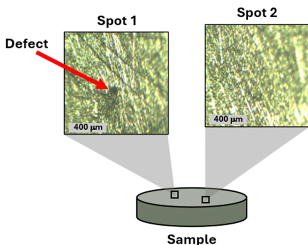
Fig. 3 Schematic of spot 1 and spot 2 found on 0.4% wt carbon sample with corresponding images from confocal Raman spectrometer. Spot 1 shows a significant defect and spot 2 does not, presumably this leads to their varying Raman spectra. The scale bar for each spot represents 400 \mu\text{m} .
