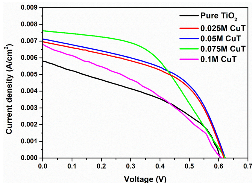
Fig. 9 J–V analysis of pure and various Cu-doped TiO 2 DSSCs.
