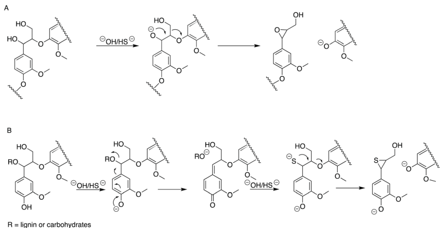
Fig. 2 Cleavage of non-phenolic and phenolic \beta -O-4' bonds during kraft pulping. (A) Slow sulfur-independent reaction, endo -depolymerisation; (B) fast sulfur-dependent reaction, exo -depolymerisation. 7,8 Reproduced from ref. 5 with permission from Wiley, copyright 2023.
