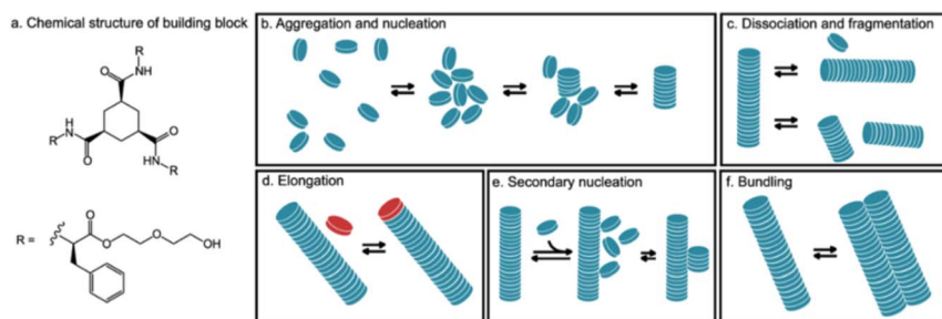
Fig. 5 The chemical structure of the 1,3,5-cyclohexanetricarboxamide used in this sturdy, and the different types of self-assembly processes and nucleation pathways studied in this contribution and presentation. Reproduced from https://doi.org/10.1039/D4FD00188E with permission from the Royal Society of Chemistry.
