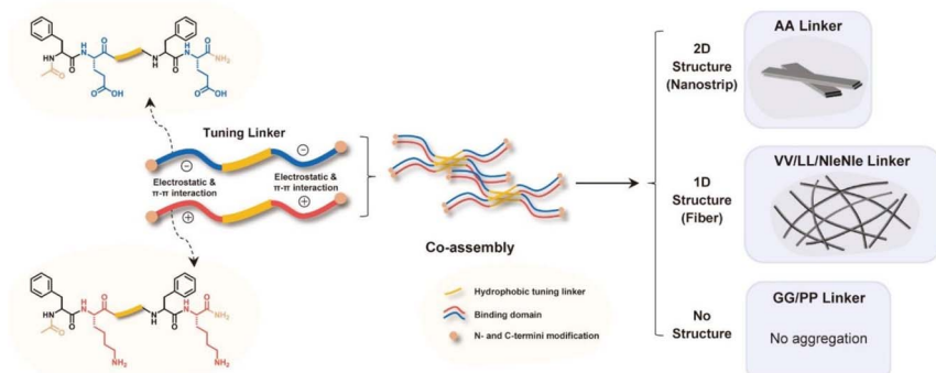
Fig. 1 The effects of oppositely charged peptides containing different linkers on the self-assembly structure. Reproduced from https://doi.org/10.1039/D4FD00209A with permission from the Royal Society of Chemistry.
