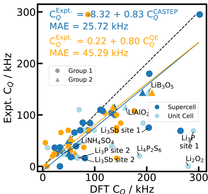
Fig. 4 Reference scale for ^7\text{Li} C_Q . The ^7\text{Li} C_Q values for 23 Li-containing compounds are calculated with PBE, fixed cell geometries, using CASTEP for unit cells (light blue), 2 \times 2 \times 2 supercells (blue), and Quantum ESPRESSO (orange) with the default PP in each case. The experimental values from literature can be found in ESI Table S4.† The dashed diagonal line indicates the limit of ideal correlation. Outliers including \text{Li}_3\text{P} and \text{Li}_3\text{Sb} are labelled and described further in the text. The data point for \text{Li}_3\text{N} [site 1] ( C_Q = 582 kHz, ESI Table S4†) is beyond the depicted range, but is included in the regression analysis.
