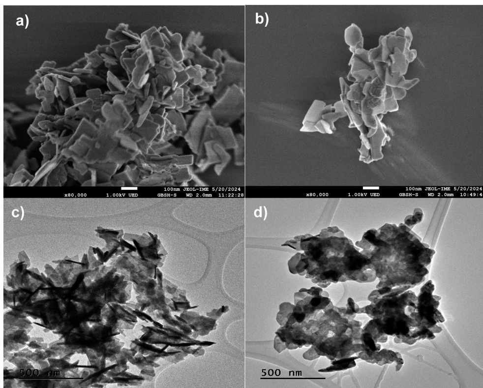
Fig. 4 FESEM images of a) \text{Bi}_2\text{O}_2\text{CO}_3 and b) Chol10% \text{Bi}_2\text{O}_2\text{CO}_3 . TEM images of c) \text{Bi}_2\text{O}_2\text{CO}_3 and d) Chol10% \text{Bi}_2\text{O}_2\text{CO}_3 .
