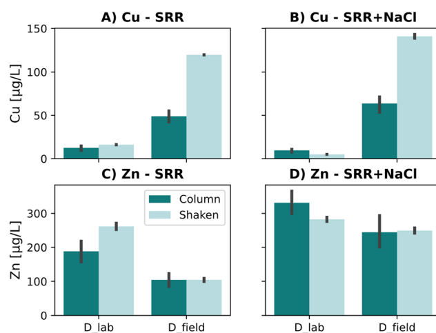
Fig. 5 Comparison of the Cu (A and B) and Zn (C and D) concentrations [μg L -1 ] depending on the SRR leached from the sorptive filter media of SCM-D prestressed in situ or in the lab with the quiescent column (only timestep 4 h and 48 h) and shaken batch extraction procedures (DIN 19529).
