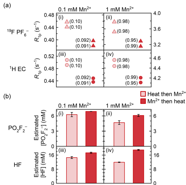
Fig. 7 (a) ^{19}\text{F} ( \text{PF}_6^- ) (triangles) and ^1\text{H} (EC) (circles) longitudinal paramagnetic relaxation rates ( R_{1\rho} ) and (b) estimated concentrations of \text{PO}_2\text{F}_2^- and HF in electrolyte solutions to which \text{Mn}^{2+} was added before (red) or after heating (pink) at 60 °C for ten weeks. Values next to the relaxation data indicate the Mn concentration in mM measured by ICP-OES. \text{PO}_2\text{F}_2^- estimated concentrations were derived from integrating ^{19}\text{F} spectra relative to \text{PF}_6^- (assuming 1 M \text{PF}_6^- ); HF estimated concentrations were derived from ^{19}\text{F} spectra as well as from ^1\text{H} spectra relative to EC (assuming 4.5 M EC). Electrolyte solutions comprised 1 M \text{LiPF}_6 in 3 : 7 EC : EMC (v/v), to which 0.1 or 1.0 mM \text{Mn}(\text{TFSI})_2 was added.
