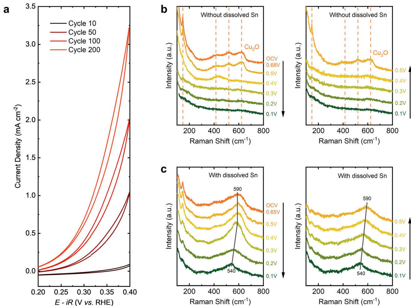
Fig. 4 (a) Cyclic voltammetry on Cu disk in Ar-saturated 1 M KOH + 50 mM \text{Sn(OH)}_3^- at 10 \text{ mV s}^{-1} and 800 rpm. (b) In situ EC-Raman spectra on Cu nanoparticle electrode in Ar-saturated 4 M KOH. (Left) Polarization in the cathodic direction from pristine electrode. (Right) Subsequent polarization in the anodic direction. (c) In situ EC-Raman spectra on Cu nanoparticle electrode in Ar-saturated 4 M KOH and 0.1 M \text{Sn(OH)}_3^- (prepared with 4.1 M KOH and 0.1 M SnO). (Left) Polarization in the cathodic direction from pristine electrode. (Right) Subsequent polarization in the anodic direction. The electrode is scanned and held at each potential (vs. RHE) for at least 2 min before taking Raman measurements. Orange dashed lines: \text{Cu}_2\text{O} reference bands. 43,44 Gray solid lines: band assigned to surface \text{Sn(OH)}_x (guides to the eye).
